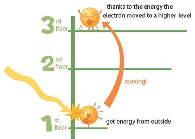
fig.5: energy level change of electrons
