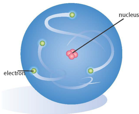
Fig.1: atomic structure
